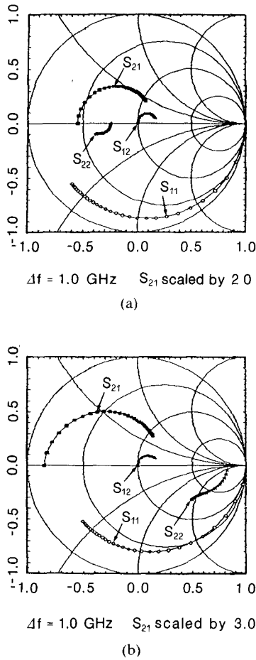
Fig. 3. Simulated scattering parameters with respect to 50\ \Omega for the same device as in Fig. 2(a)–(e). 1 and 2 stand for gate and drain electrodes, respectively. Distributed gate effects are included. The source and gate voltages are V_s = 0 , V_g = 0 V for all working points. (a) V_d = 0.5 V (linear region); (b) V_d = 3.0 V (saturation). The frequency spacing between points is 1 GHz.
