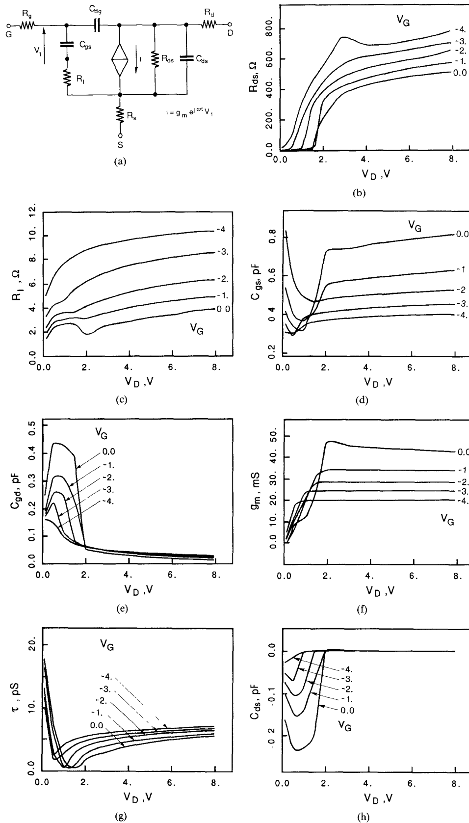
Fig. 4. (a) Small-signal equivalent circuit. Variation of small-signal parameters as a function of working point: (b) R_{ds} , (c) R_f , (d) C_{gs} , (e) C_{gd} , (f) g_m , (g) \tau , and (h) C_{ds} . R_d and R_s are almost constant and can be assumed to take on the average values R_d = 7 \Omega , R_s = 2.5 \Omega .
