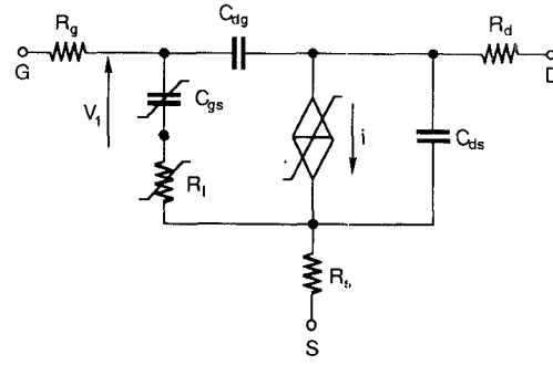
Fig. 5. Large-signal model derived from the small-signal model of Fig. 4(a). One has i(t) = f[v_1(t - \tau), v_2(t)] , C_{gs} = C_{gs}(v_1) , R_I = R_I(v_1) .
